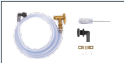
Universal Hose Set 3/4 inch Kit for complete water extraction and water level display for above-ground rainwater storage tanks. Consisting of 2.15 m (7' 0.6 inch) flexible hose, extraction tap and various connection options. Suited to all storage tanks. order no. 220015
