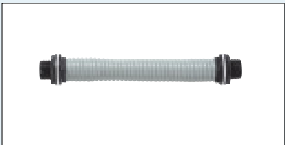
Water butt connection kit Consisting of two hose connections with lock nut and 25 cm (9.8 inch) hose. 19 mm (3/4 inch) order no. 504017
